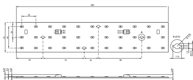
Fortimo LED Line 1ft 650lm 840 3R HV2
