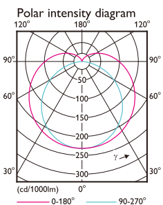
1 x TLED 18W 4000K/6500K
