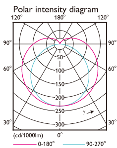
1 x TLED 9W 4000K/6500K
