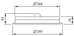
RC360BW60L60 Afmetingen in mm.
