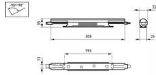
BCX422 2700 HE L305 CE/CCC Afmetingen in mm.
