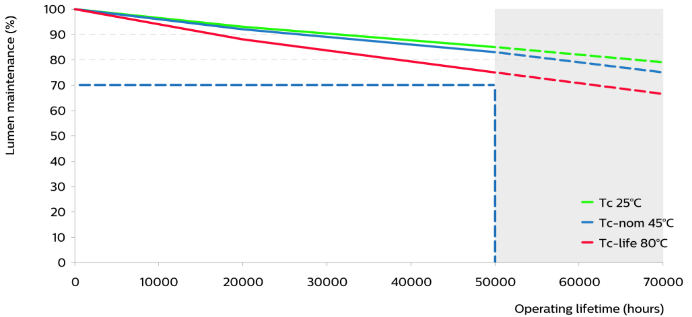
Lumen maintenance for B50 at current I-life conditions
