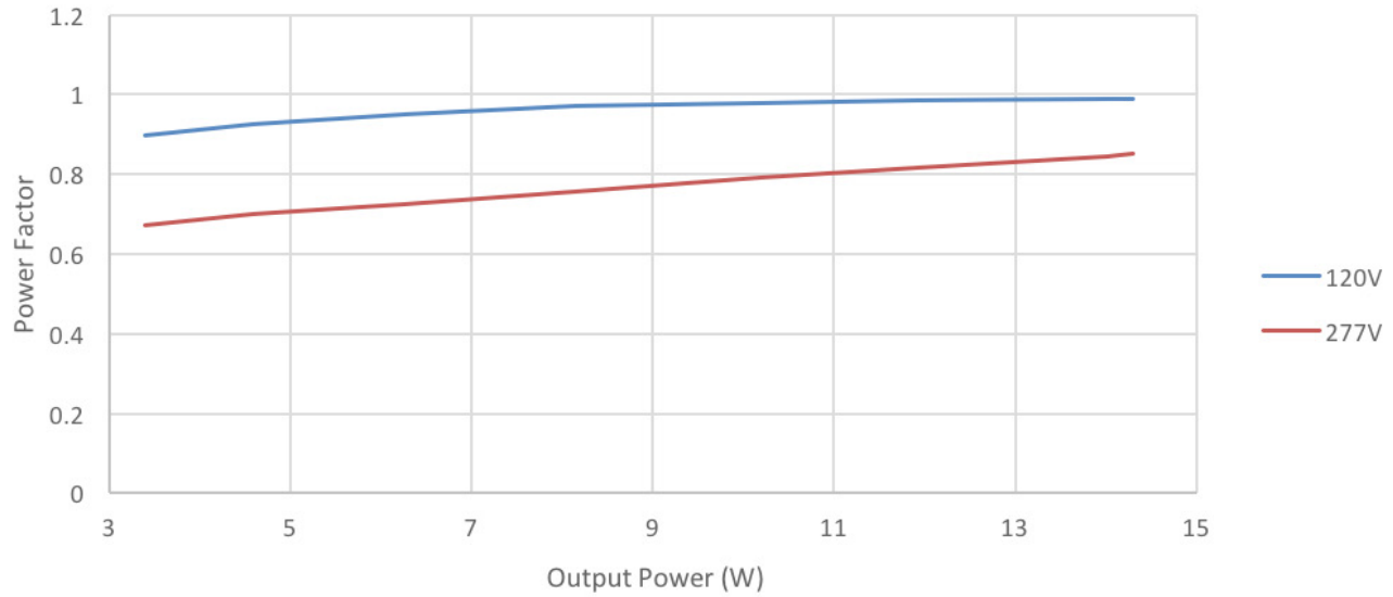
Output Power Vs. PF_350mA
