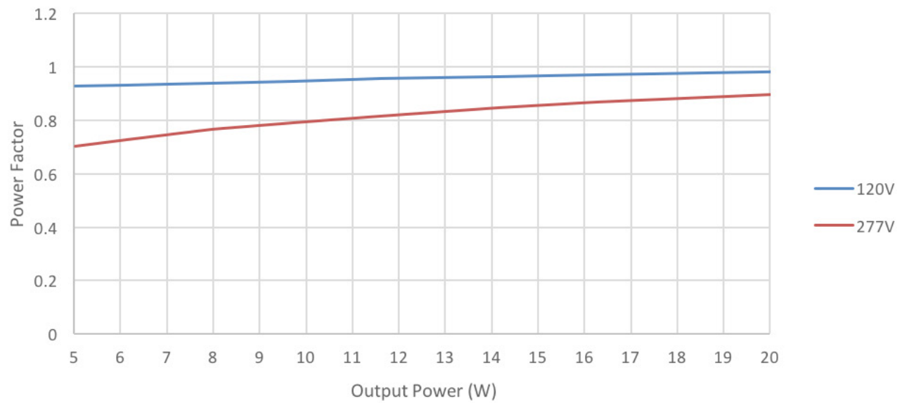
Output Power Vs. PF_500mA
