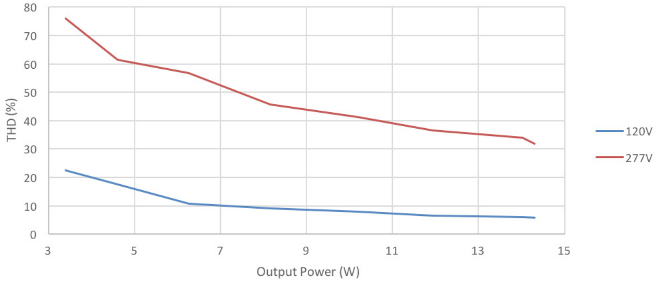
Output Power Vs. THD_350mA
