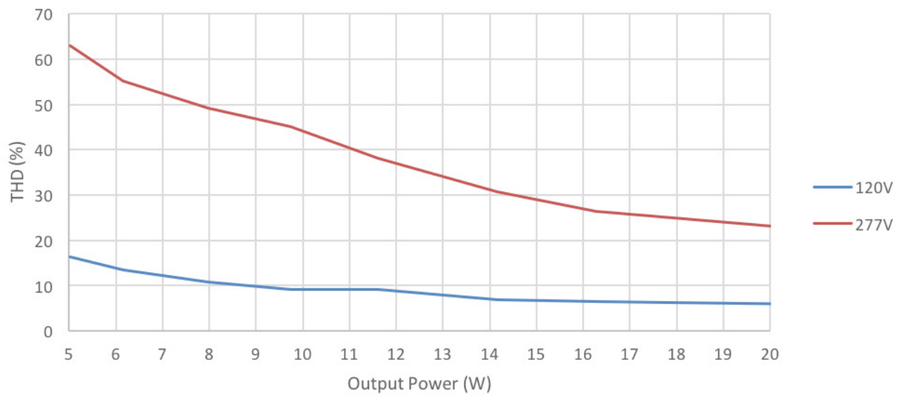
Output Power Vs. THD_500mA
