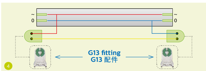
4 Re-wire the batten according to scheme / 按图对灯具进行重新布线
