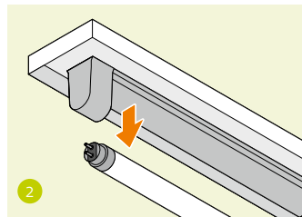
2 Remove all existing FLUORESCENT TUBES from luminaire 拆除灯具上的全部现有荧光灯管
