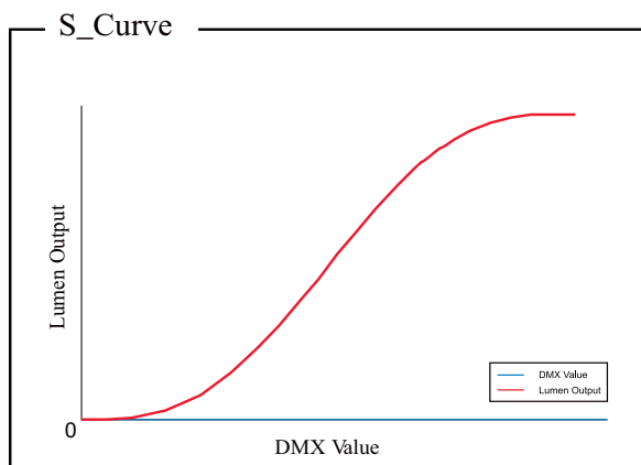
Figure 10: 200F TV Fresnel LED Luminaire Dimmer Curves
