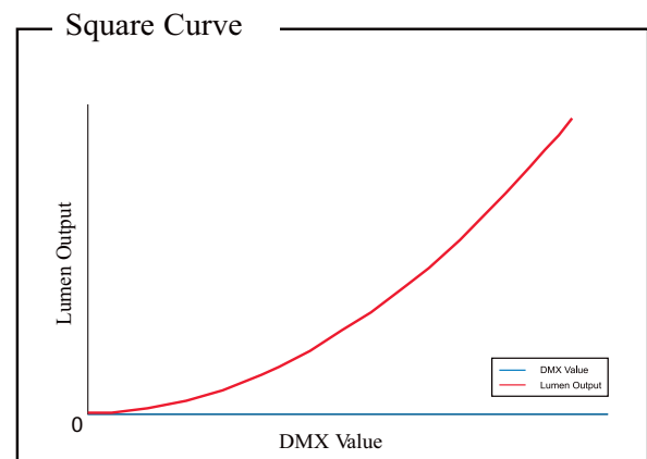
Figure 10: 200F TV Fresnel LED Luminaire Dimmer Curves
