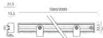
WALL MOUNTED
