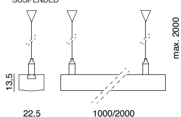
SUSPENDED
