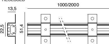
RECESSED
