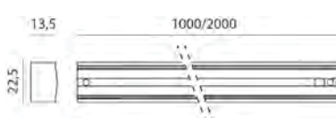
RECESSED
