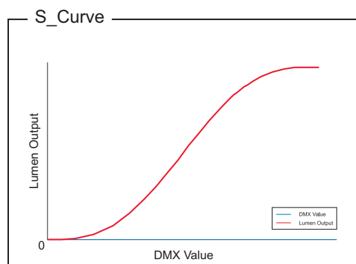
Figure 9: SL BAR 660 RGBW LED Luminaire Dimmer Curves
