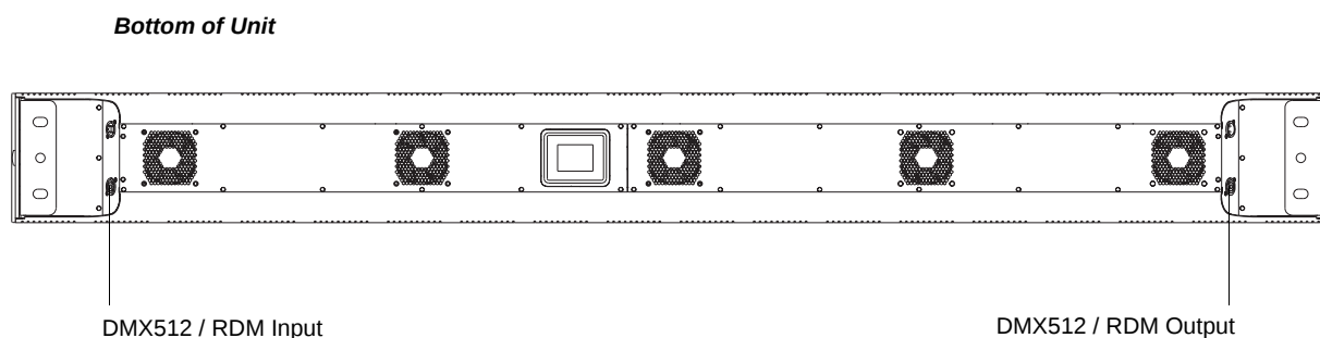
Figure 5: SL BAR 660 RGBW LED Luminaire DMX512 Input / Output Connections
