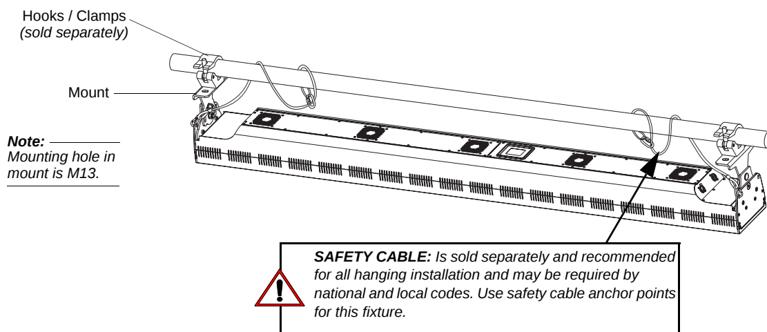
Figure 7: Mounting Luminaire - Hanging Applications
