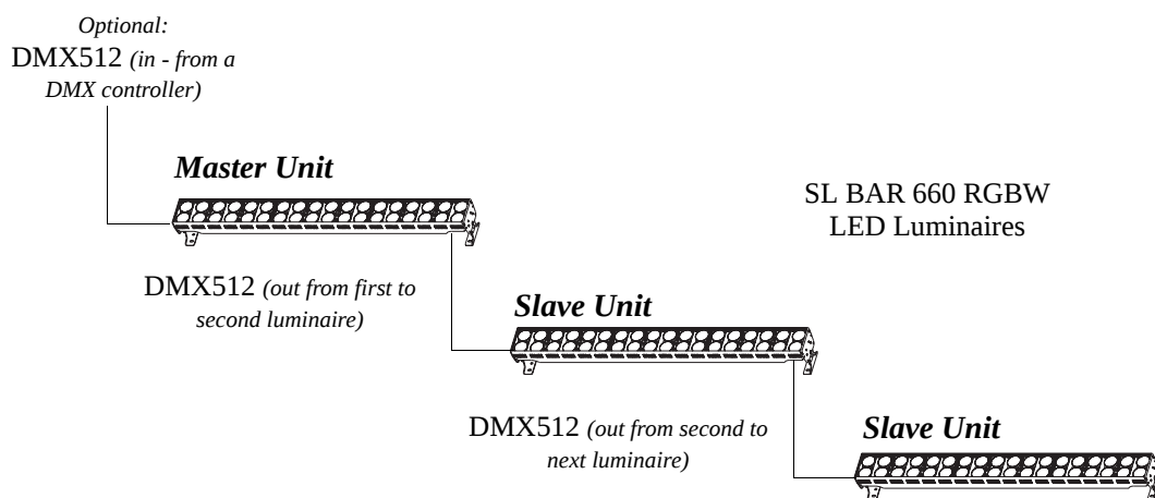
Figure 10: SL BAR 660 RGBW LED Luminaire - Master / Slave Configuration
