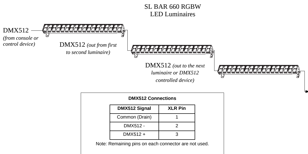
Figure 6: SL BAR 660 RGBW LED Luminaire - DMX512 Connections
