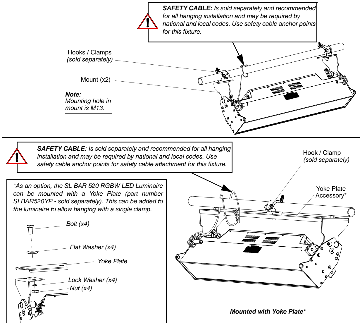
Figure 7: Mounting Luminaire - Hanging Applications
