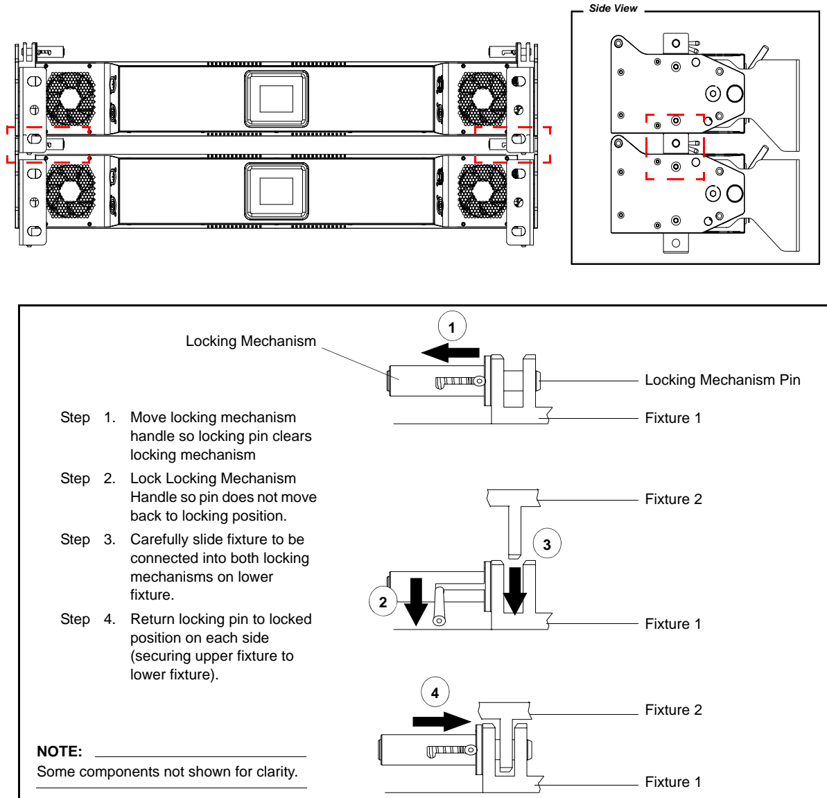
Figure 8: Connecting Luminaires Top-to-Bottom
