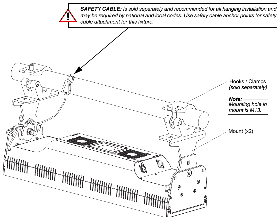
Figure 7: Mounting Luminaire
