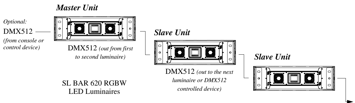
Figure 10: SL BAR 620 RGBW LED Luminaire - Master / Slave Configuration
