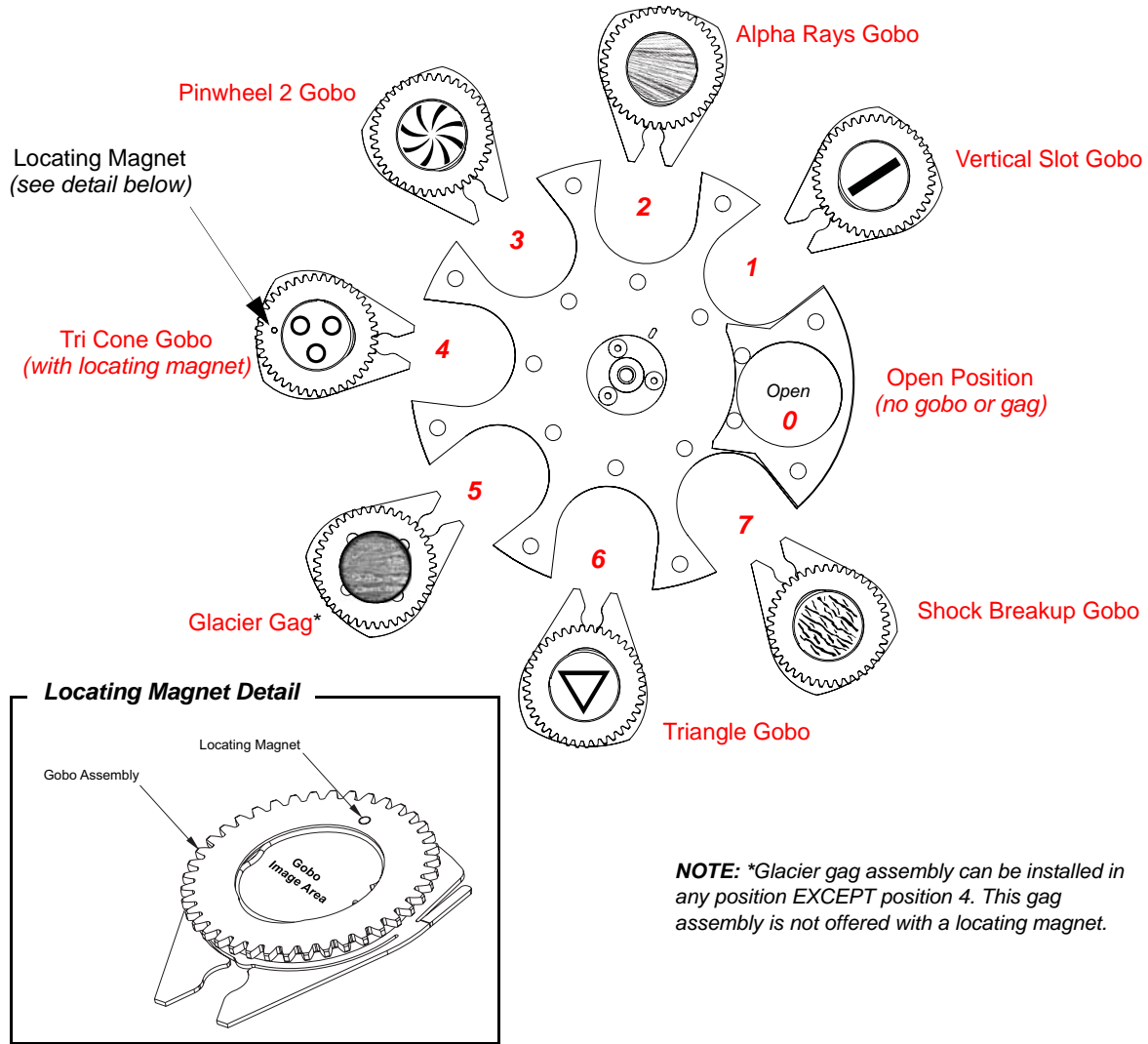
Figure 1: Standard Gobo Load for VL440/770/880 Rotating Gobo Wheel
