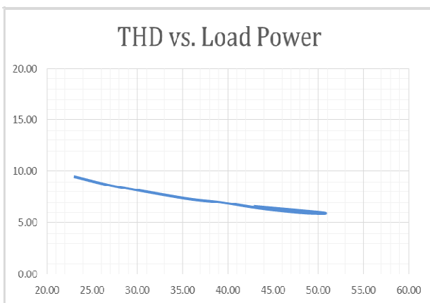
THD vs Load Power :
