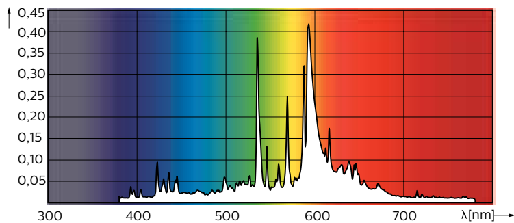
CPO-TT 60W /628
