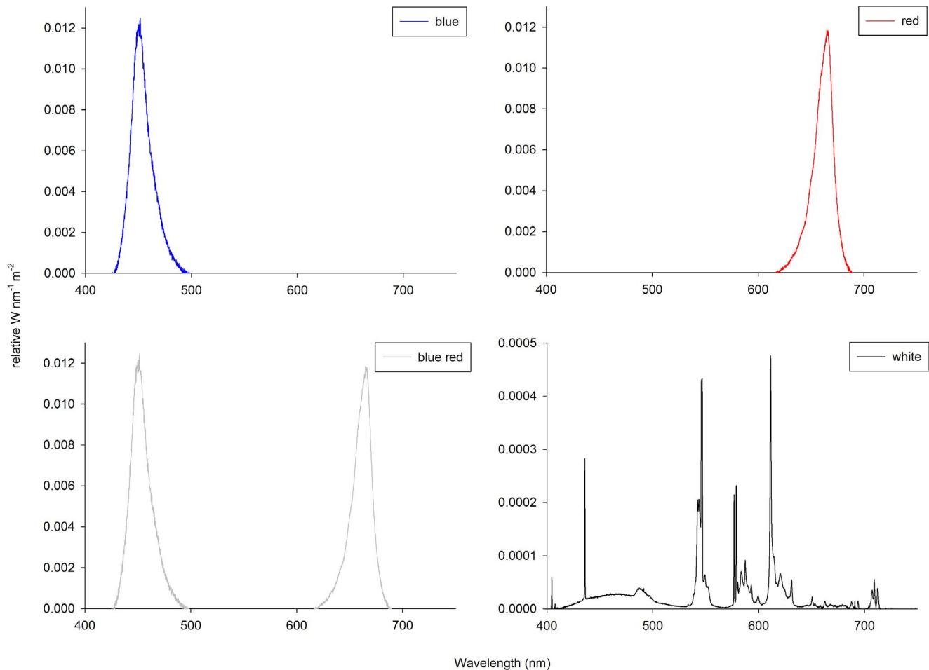
Figure 1. Spectral analysis of the LED and T5 fixtures used for the experiment, representative for both irradiance levels used. doi:10.1371/journal.pone.0092781.g001
