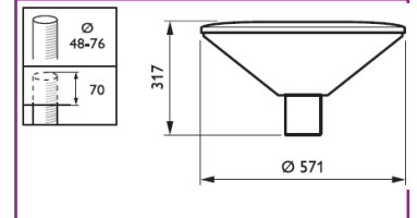
TownGuide BDPI02 afmeting in mm
