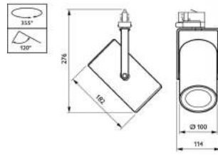
GreenSpace Accent Projector ST320T Afmetingen in mm.
