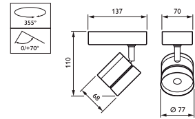
ST120C LED8S Afmetingen in mm.
