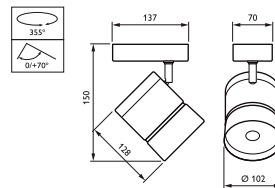
ST120C LED24S Afmetingen in mm.
