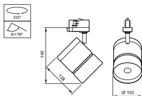
ST120T LED24S Afmetingen in mm.
