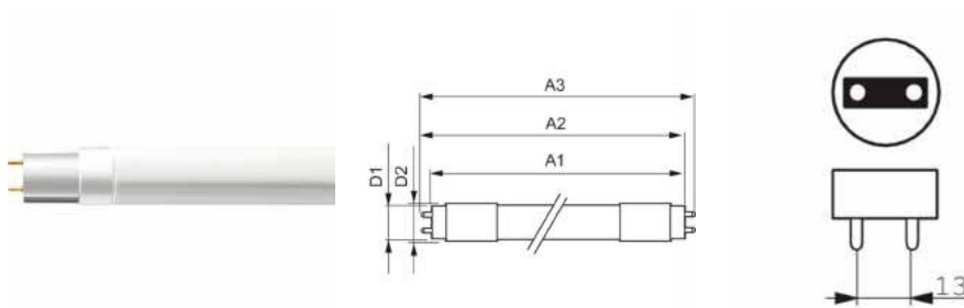
CorePro LEDtube (EM/MAINS)
