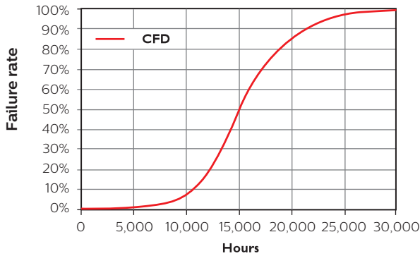
Failure rate curve of CorePro LEDspot MV GU10
