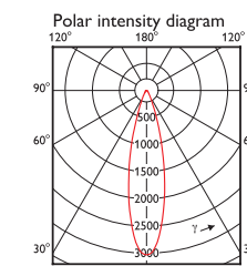
15-75W AR111 2700K 40D
