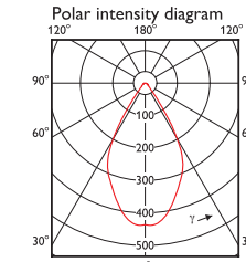
5-50W GU10 2700K 36D
