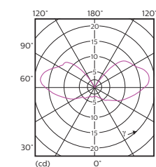
1.2-10W G4 2700K
