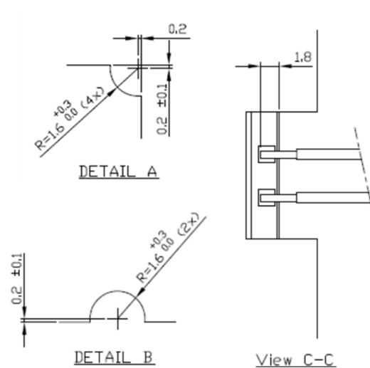
Figure 5: Details A and B (screw openings) and view C-C (solder orientation on PCB) of Figure 4 –integration level 2
