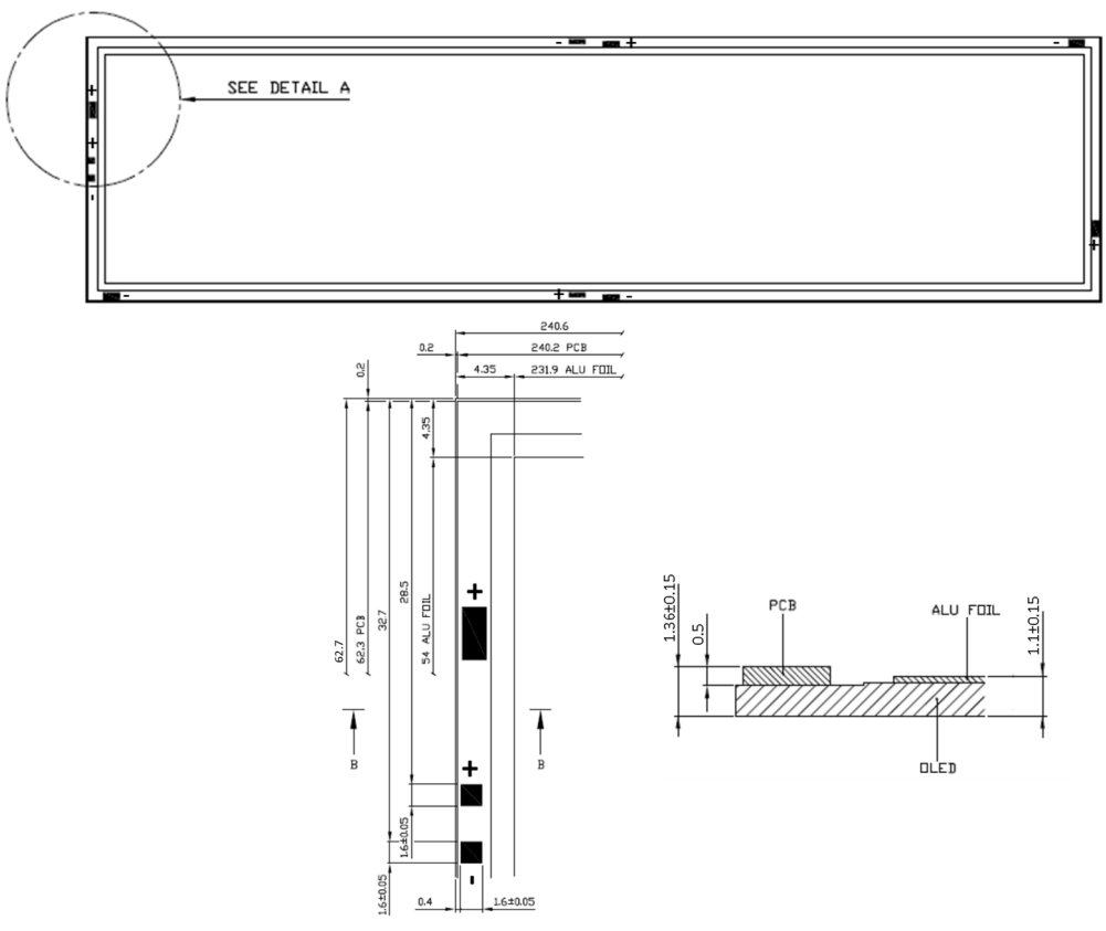
Figure 5.2: Brite FL300 L ww N w/o Rset – rear view, integration level I (top); Detail A (left) and cross section B-B (right)
