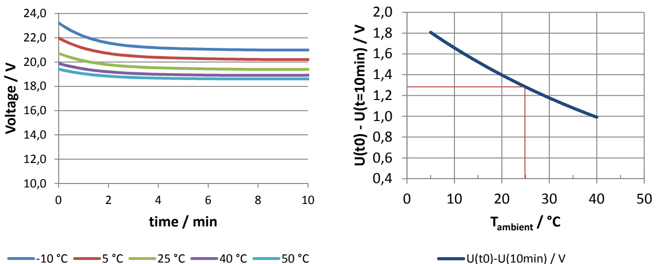
Figure 13 – (left) dependency of driving voltage at constant current ( I = 0.368 A) on ambient Temperature T_{ambient} ; (right) voltage drop after turn on at T_{ambient} = RT (= 25 °C)
