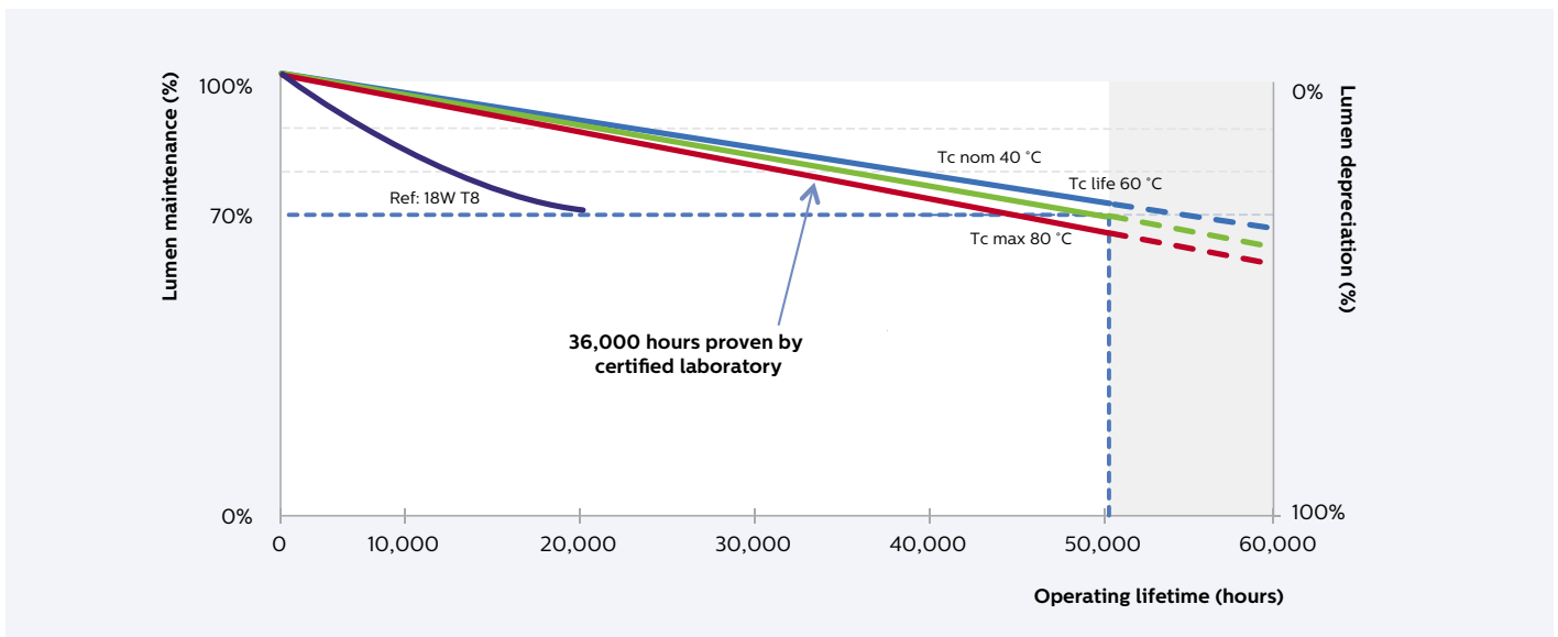
Lumen depreciation as a function of operating hours for LED Strip 1 ft 650 lm LV3 at different Tc values.
