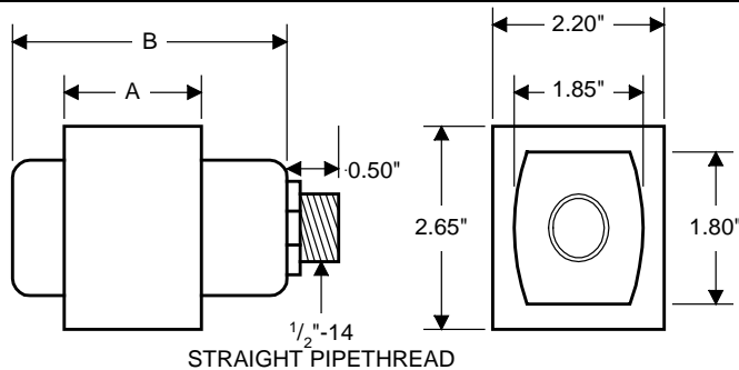
Fig. 11 J-Box Ballast
