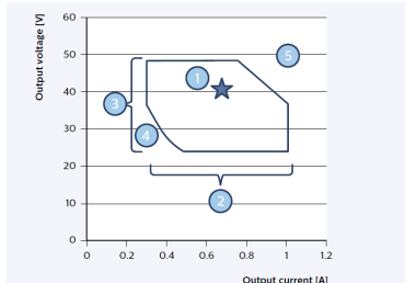
Figure 15. Example operating window of the Xitanium Driver (36W in this case)
