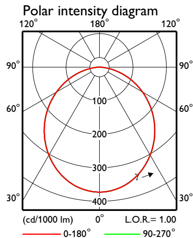
Figure 4. Light distribution diagram
