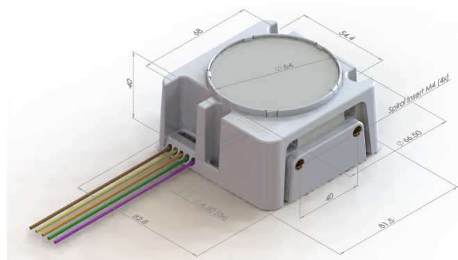
Figure 3B. Fortimo LED DLM Flex Module dimensions
