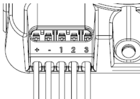
Figure 12. Connection to the module
