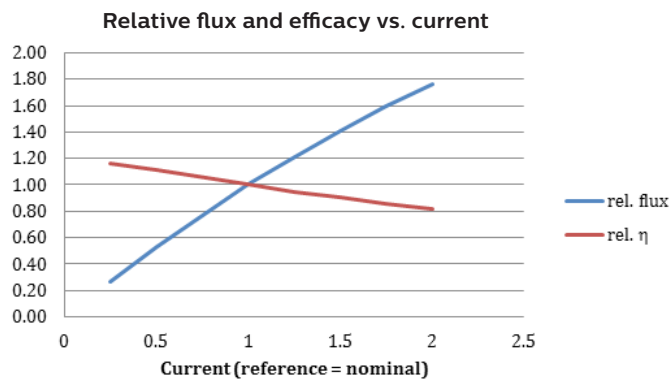
Figure 14. Example graph showing flux and efficacy as a function of current
