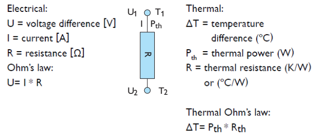
Figure 10. Electrical and thermal analogy
