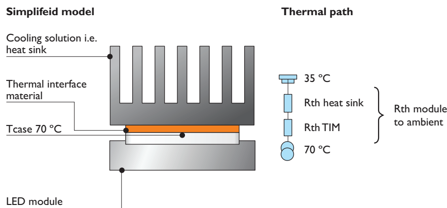
Figure 11. A simplified model of the thermal path from LED module to ambient
