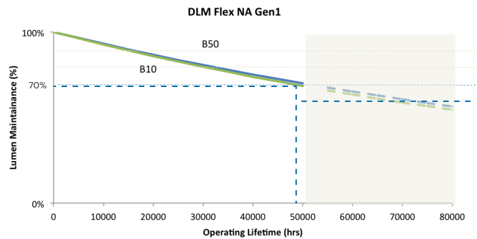
Figure 5. Example lumen maintenance as a function of operating hours for B10 and B50 at Tc nominal
