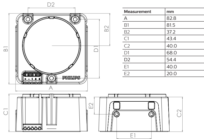
Figure 3A. Fortimo LED DLM Flex Module dimensions
