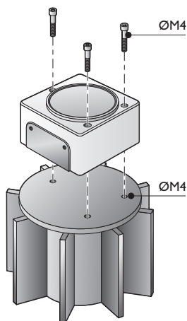
Figure 6. Screw installation
