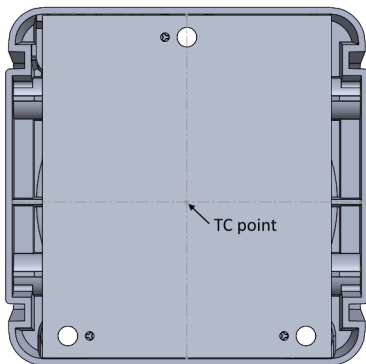
Figure 7. Temperature test point T_c
