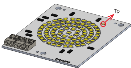
Figure 8. Tp temperature measurement point
