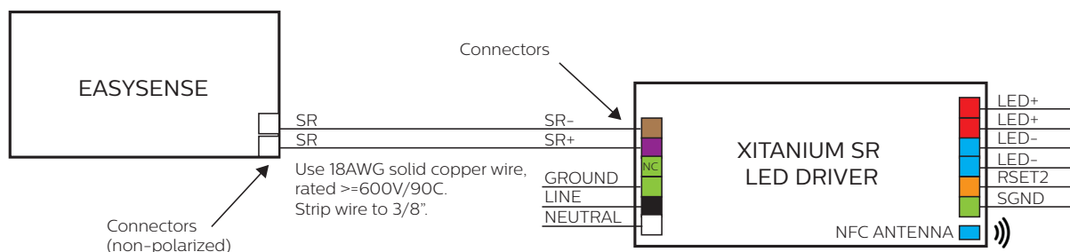
Figure 12. Wiring diagram with Philips Advance SR driver.
