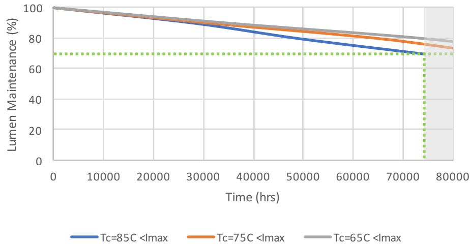
Lumen Maintenance
