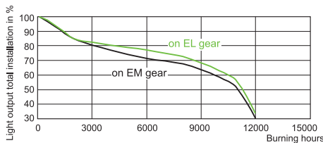
CDM-T 150W /942 on electronic & electromagnetic gear
