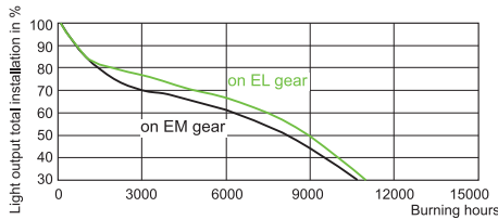
CDM-T 35W /830 on electronic & electromagnetic gear
