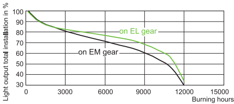
CDM-T 70W /830 on electronic & electromagnetic gear
