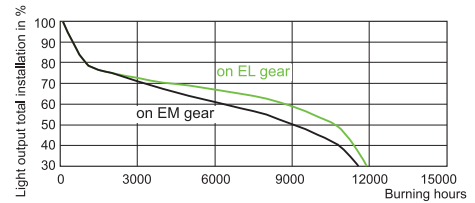
CDM-T 150W /830 on electronic & electromagnetic gear
