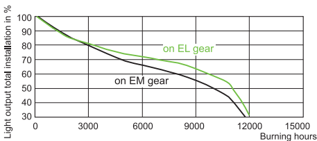
CDM-T 70W /942 on electronic & electromagnetic gear
