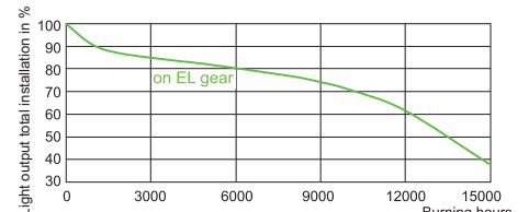
CDM-T 20W /830 on electronic gear
