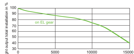
CDM-TC Elite 70W /930
