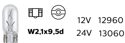
Pingão de 2W (W2,2W)
