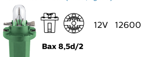
Base Plástica verde (BAX 2,0 green)
