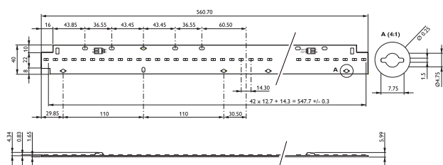
Fortimo LED Line 2ft 4000lm 830 1R HV1
