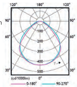
SM134V NOC
