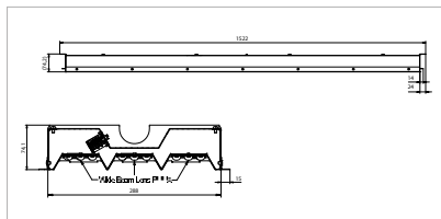
SportControl LED BCS/BPS375 Afmetingen in mm.
