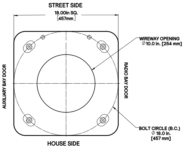
Base Plate
