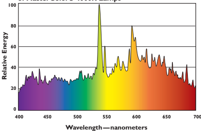
Representative Spectral Power Distribution of MasterColor® 4000K Lamps
